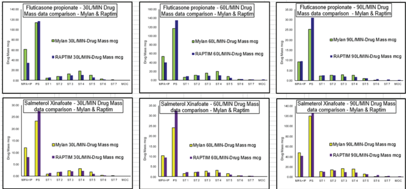
The above figure demonstrates that Raptim acquired data matches well with that acquired by Mylan, indicative of high quality of Raptim's in-vitro analysis
